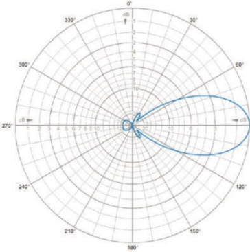
E-Plane | 405 MHz
