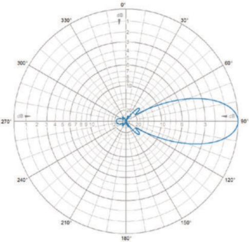
E-Plane | 405 MHz
