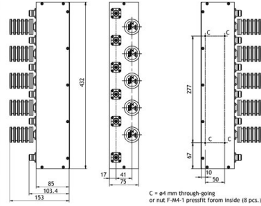
MOUNTING DETAILS_x000d_
