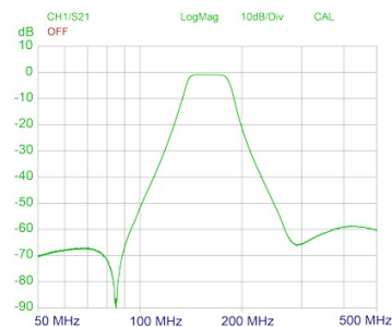
TYPICAL RESPONSE CURVE
