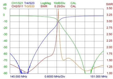
TYPICAL RESPONSE CURVES @ 4 MHz DUPLEX SPACING
