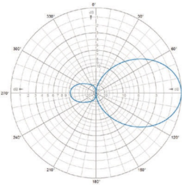
E-Plane | 72 MHz
