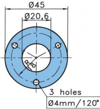
DIAGRAM INSTALLATION DETAILS
