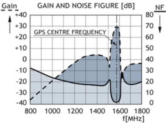
TYPICAL RESPONSE CURVES
