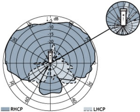
VERTICAL RADIATION PATTERN
