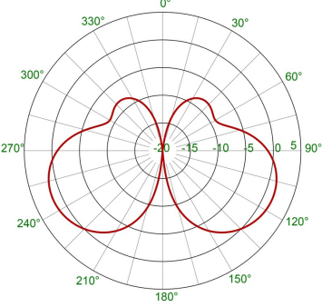
TYPICAL RADIATION PATTERN 144 MHz (E-PLANE)
