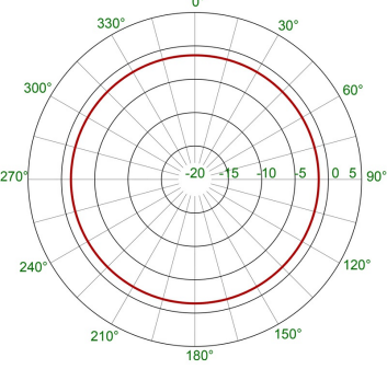
TYPICAL RADIATION PATTERN 175 MHz (H-PLANE)
