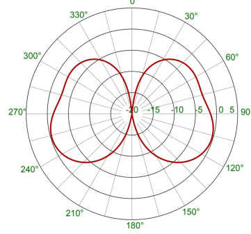
TYPICAL RADIATION PATTERN 175 MHz (E-PLANE)
