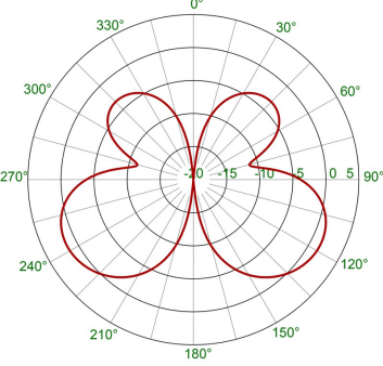
TYPICAL RADIATION PATTERN 158 MHz (E-PLANE)
