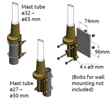
MULTI-PURPOSE MOUNTING BRACKET
