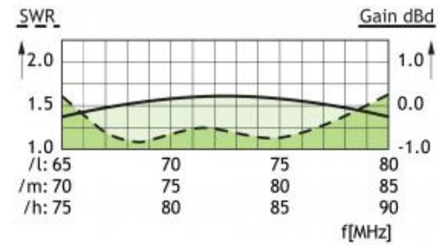
TYPICAL GAIN AND SWR CURVES
