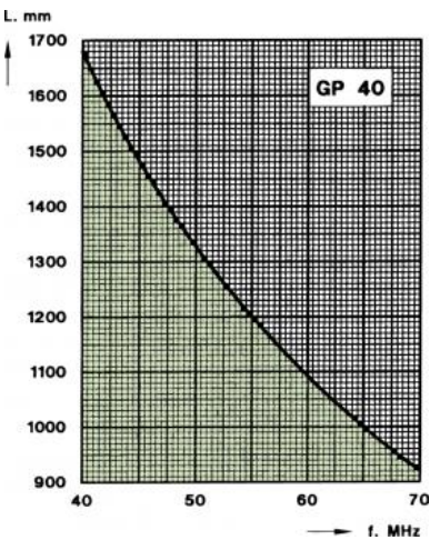
DIAGRAM CUTTING DIAGRAMS
