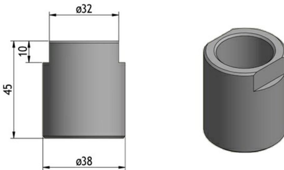
GP ADAPTOR
