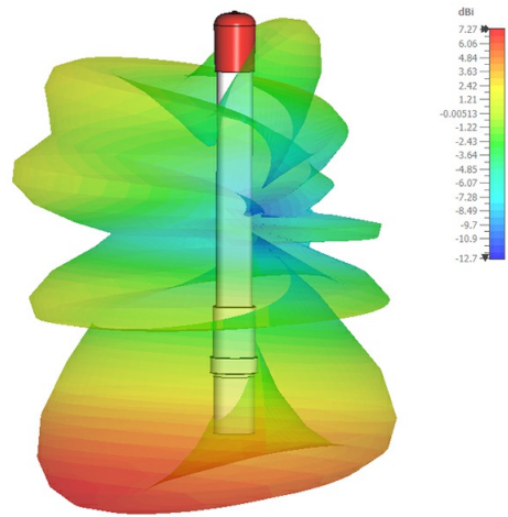
TYPICAL RADITION PATTERN (E-PLANE) FOR 3300 MHZ
