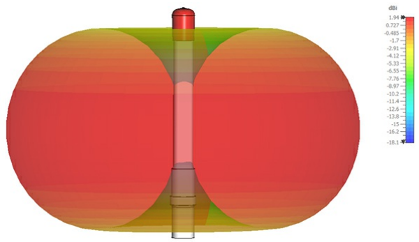
TYPICAL RADITION PATTERN (E-PLANE) FOR 710 MHZ
