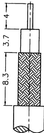
RECOMMENDED CABLE STRIPPING DIM'S (建議剝線尺寸)
