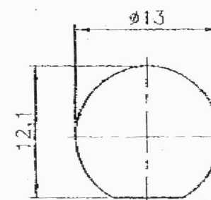
RECOMMENDED MOUNTING HOLE (建議安裝孔)
