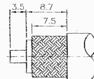
RECOMMENDED CABLE STRIPPING DIM'S (建議剝線尺寸)
