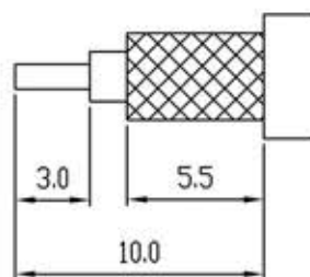
Recommend Cable Stripping
