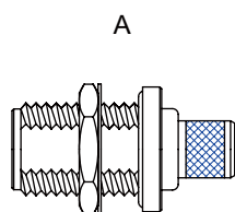
BODY+GASKET +HEX NUT +LOCK WASHER
