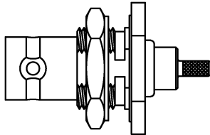
BODY + GASKET + WASHER + HEX NUT
