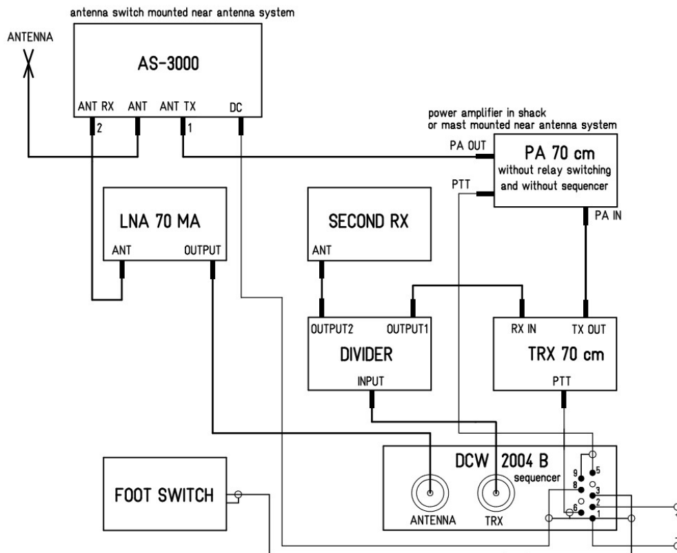
LNA 70 MA in a transmitting / receiving system with secondary receiver and a power amplifier without relay-switching.
