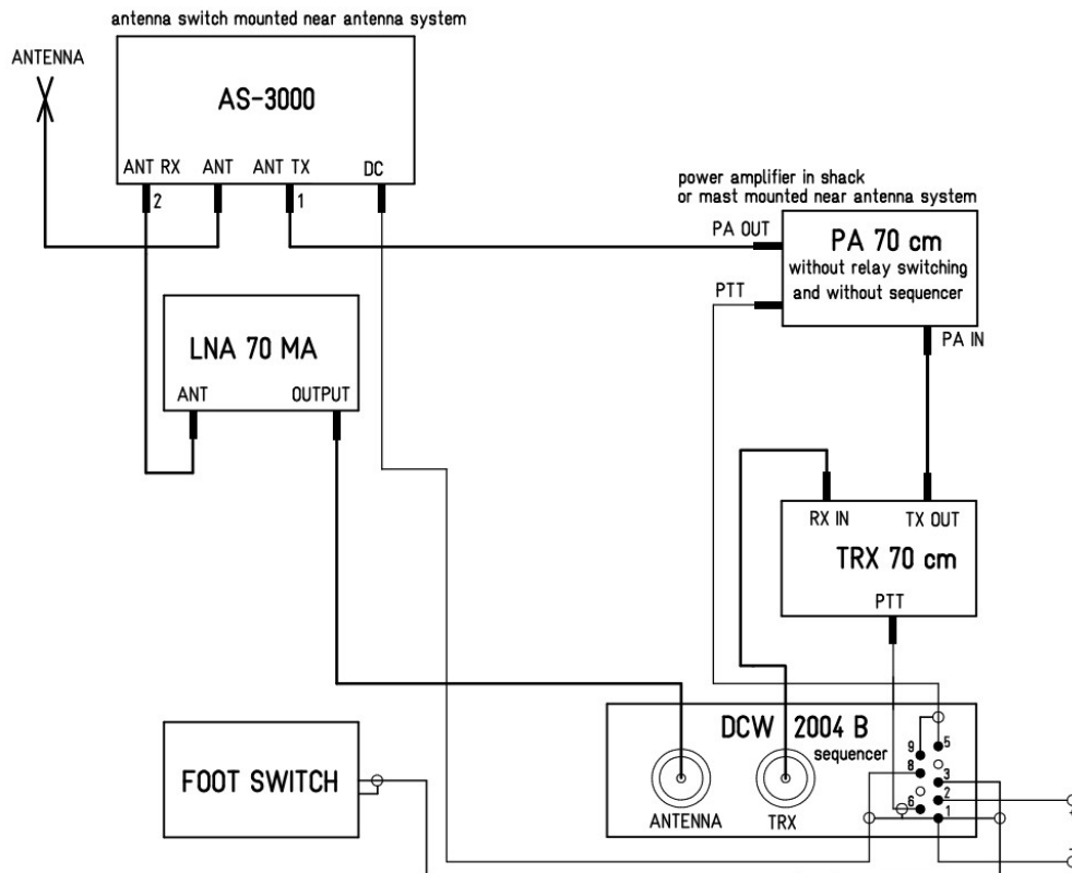
LNA 70 MA in a transmitting / receiving system with a power amplifier without relay-switching.
